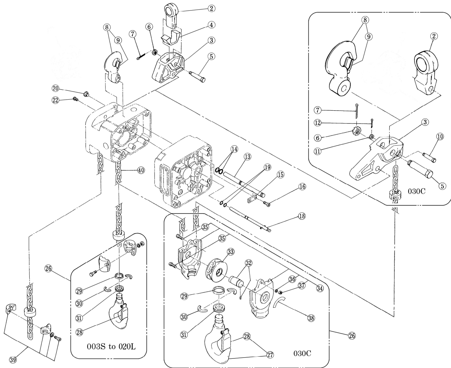
FIGURE 8-3 HOOK PARTS
